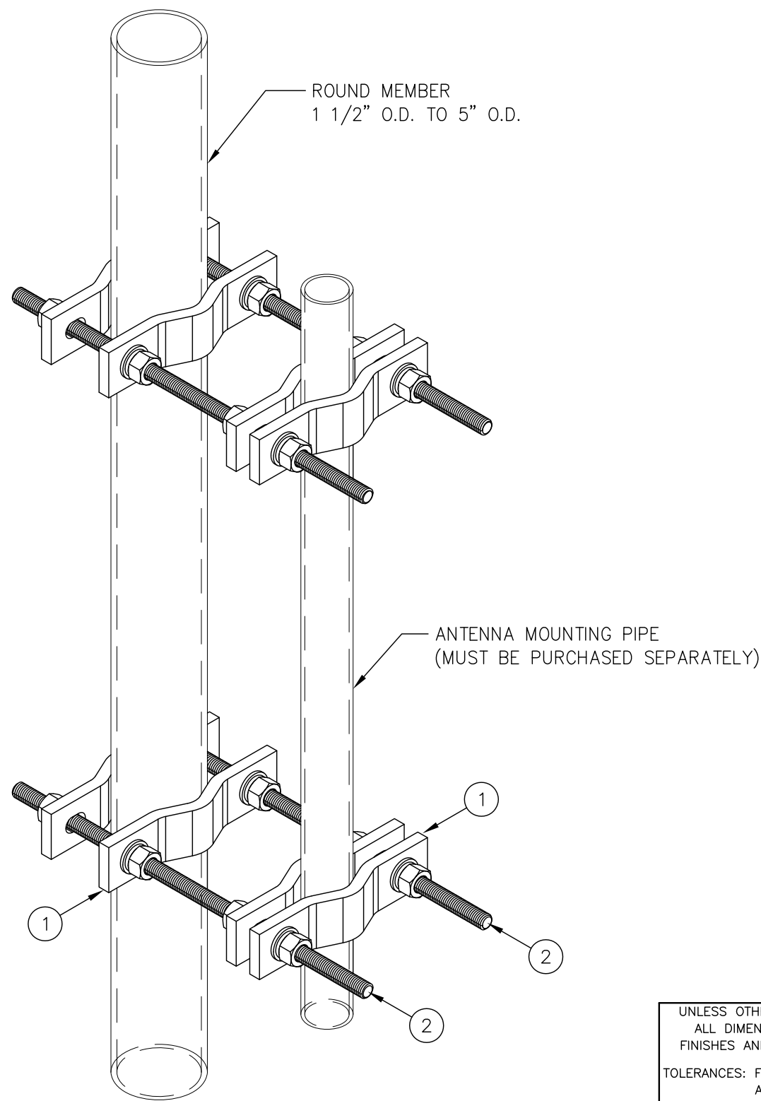
ISOMETRIC VIEW
